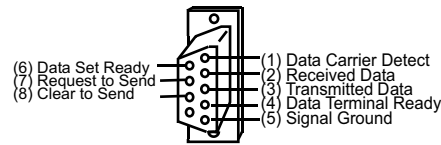
DB-9 CONNECTOR...SOCKET (female) (rear view/solder side)
