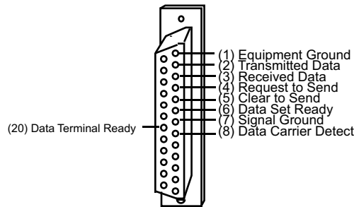
DB-25 CONNECTOR...SOCKET (female) (rear view/solder side)
